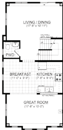
MAIN FLOOR PLAN
